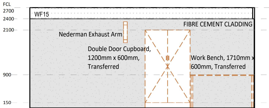
2 ELEVATION DETAIL 60-025 1 : 50
