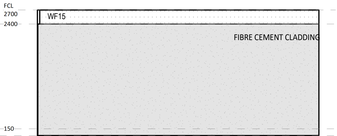
4 ELEVATION DETAIL 60-025 1 : 50
