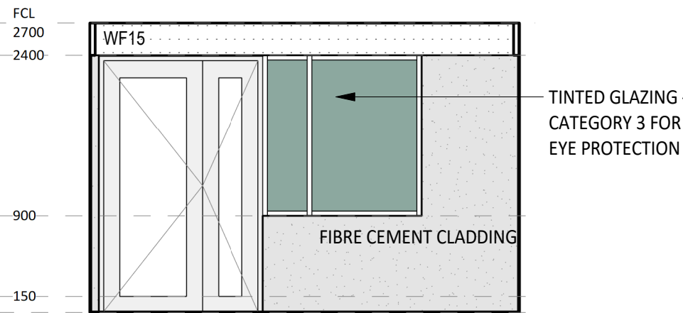
5 ELEVATION DETAIL 60-025 1 : 50
