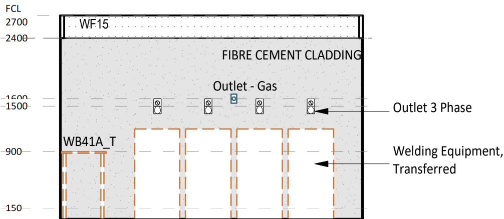
3 ELEVATION DETAIL 60-025 1 : 50
